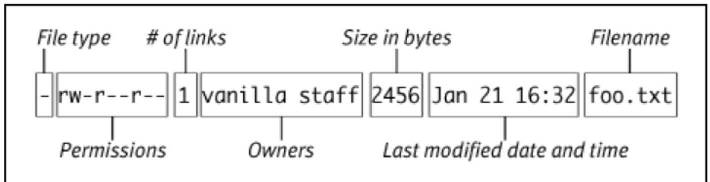
Figure 5.22. This diagram shows what the output of ls -l means.
