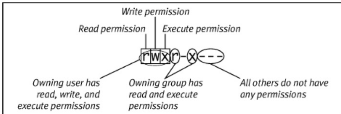
Figure 8.12. Annotated example of permission information showing the three groups of three characters indicating permissions for the user, group, and others. Permission settings: - means "no permission;" and a letter means "this permission is granted."
